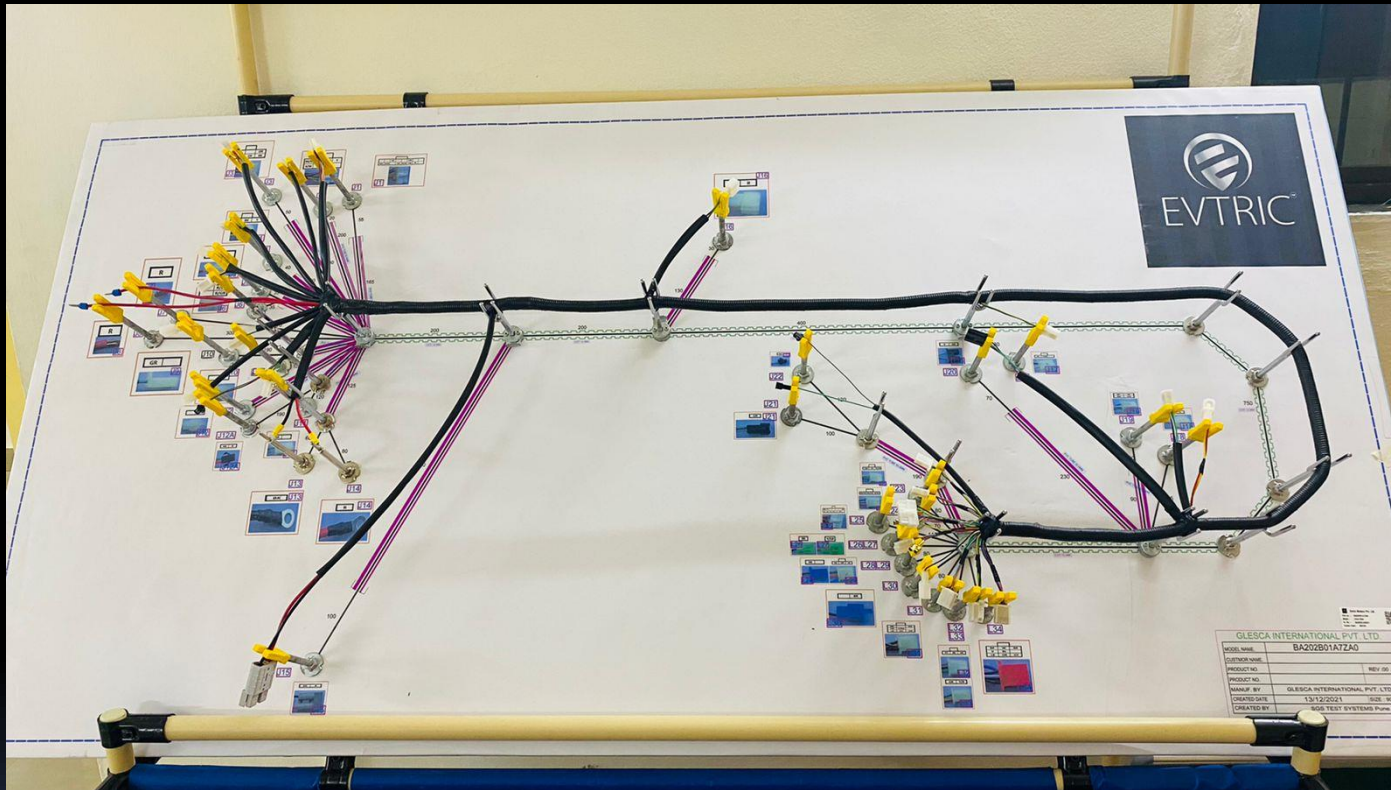
Complete Wiring Harness for Evtric Motors
